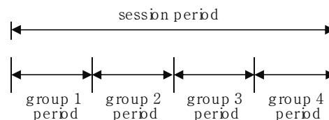
Figure 3. Session period
