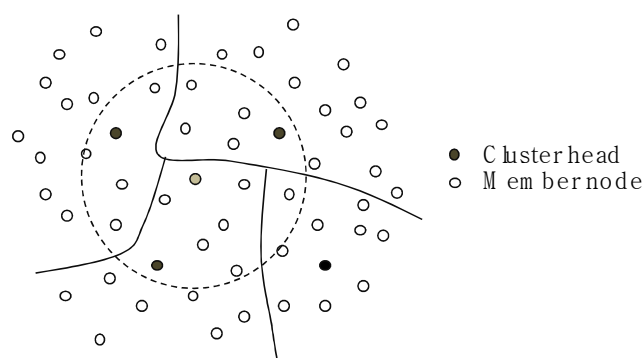
Figure 2. Clustering
