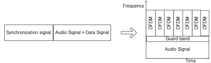
Fig. 3. Synchronization signal and data frame structure.
