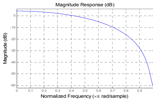
Figure 4. Magnitude response of Proakis channel B.
