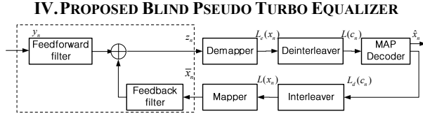
Figure 3. Block diagram of proposed blind pseudo turbo equalizer.
