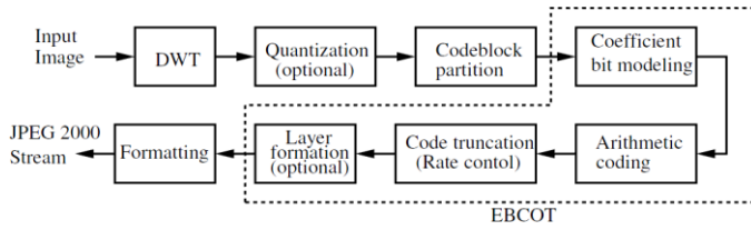
Figure 5. JPEG 2000 encoder block diagram
