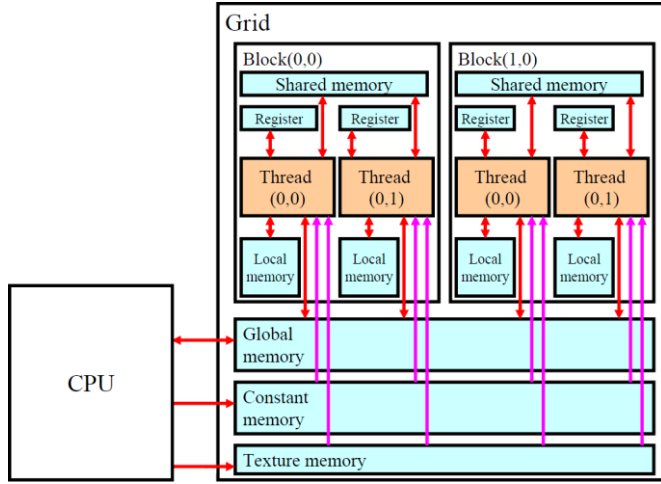
Figure 6. CUDA Architecture
