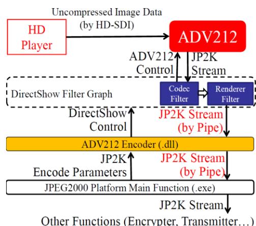
Figure 3. The architecture of ADV212 Encoder
