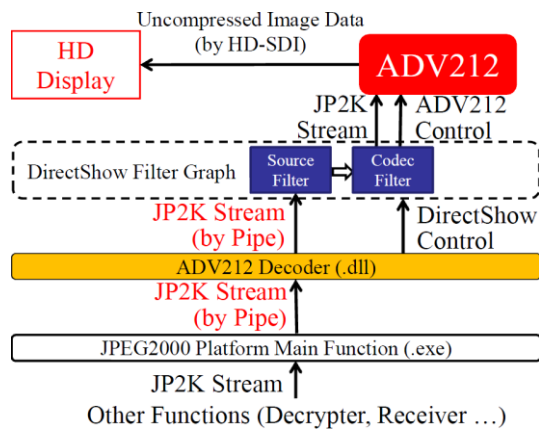
Figure 2. The architecture of ADV212 Decoder
