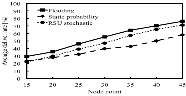
Figure 5. Message deliver rate in highway simulation scenario
