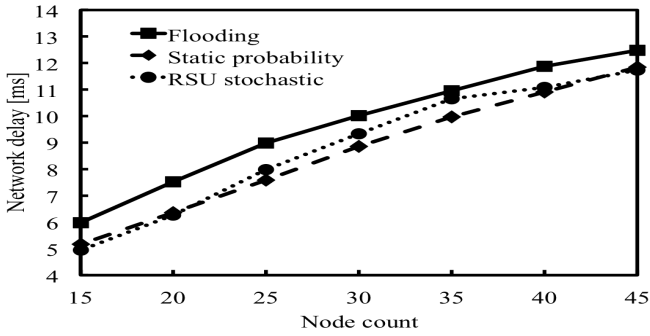
Figure 6. Delay in highway simulation scenario
