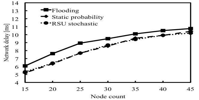
Figure 9. Delay comparison in city simulation scenario
