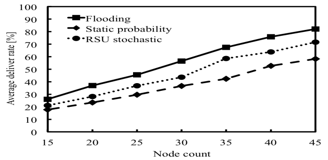
Figure 8. Message deliver rate comparison in city simulation scenario
