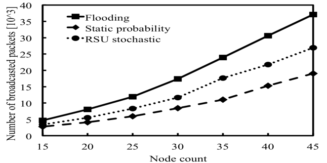
Figure 10. Packet usage comparison in city simulation scenario
