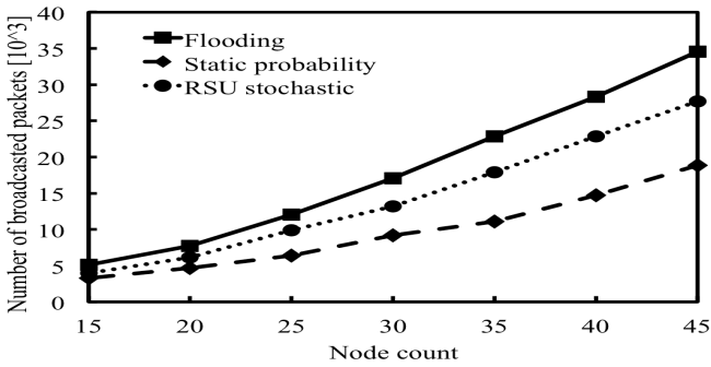
Figure 7. Packet usage in highway simulation scenario
