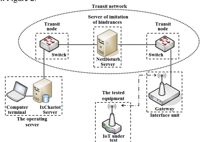
Figure 2. Block diagram of the base part model network
