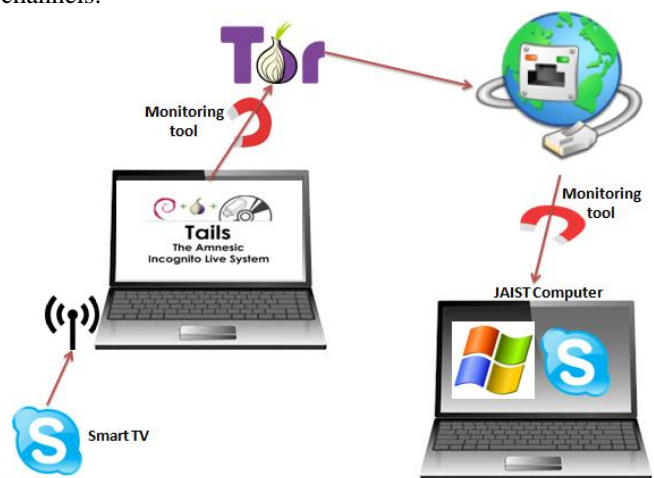
Fig. 13. Testing VoIP over TOR network
