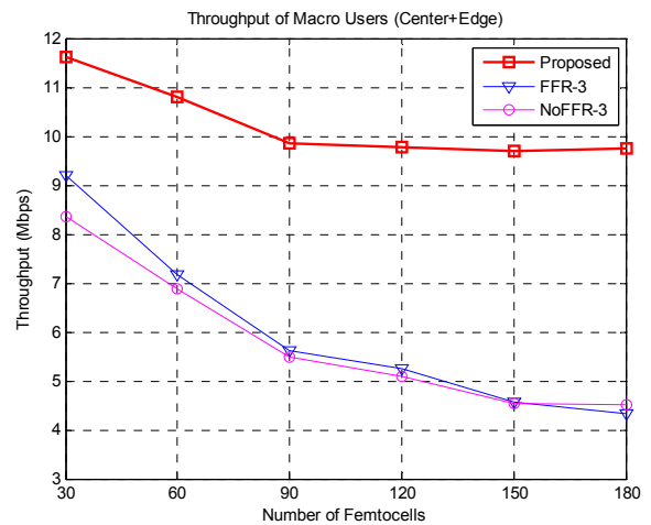
Figure 2. Throughput of macro users located in center zone and edge region as the number of femtocells varies
