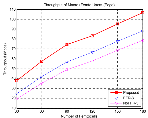
Figure 3. Throughput of macro and femto users located only in the edge region as the number of femtocells varies
